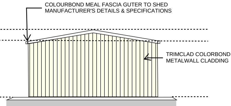
ELEVATION (WEST)
