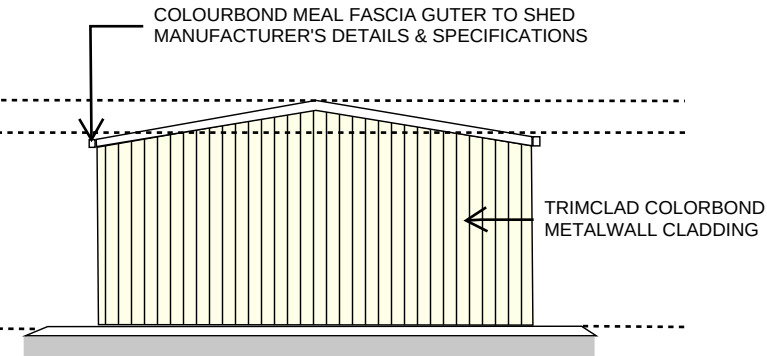
ELEVATION (EAST)
