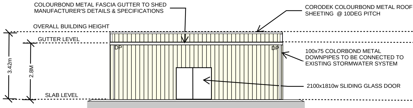
ELEVATION (NORTH)
