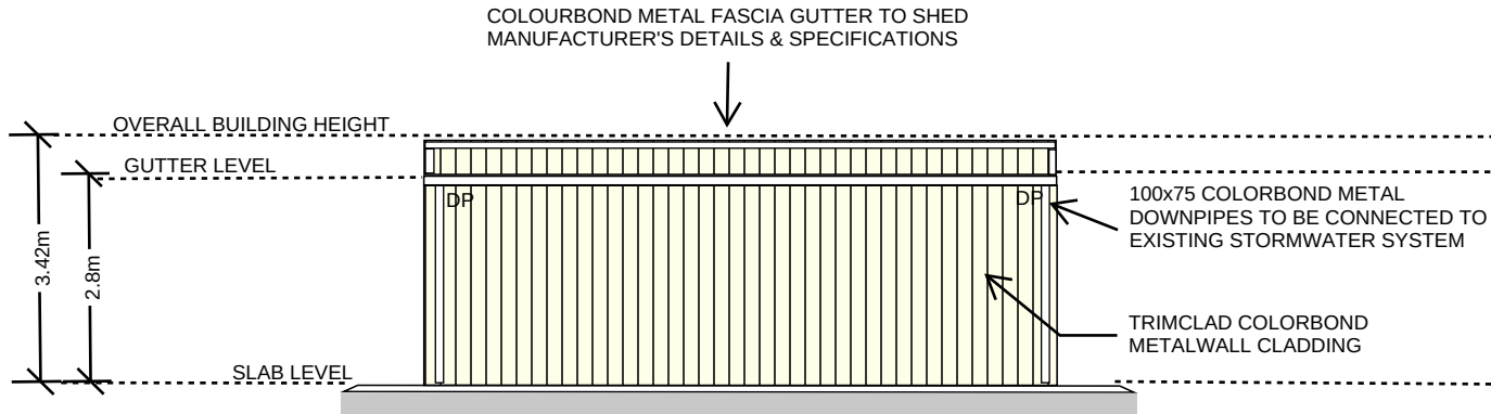
ELEVATION (SOUTH)
